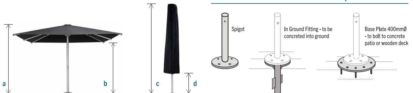
Extruded aluminium mast (strengthened)
